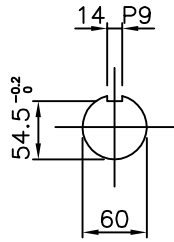
SECT. A-A
